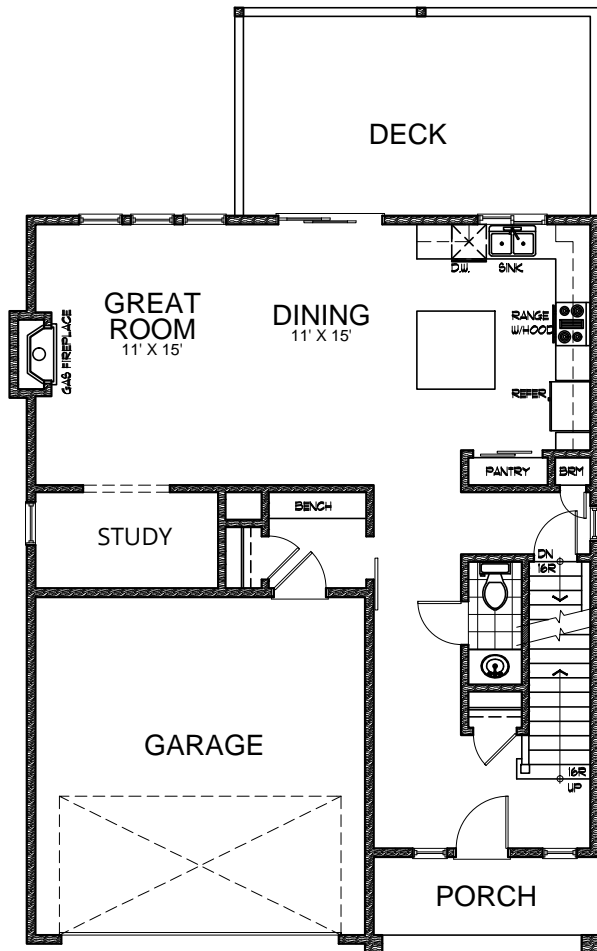
Main Floor 950 sq ft
