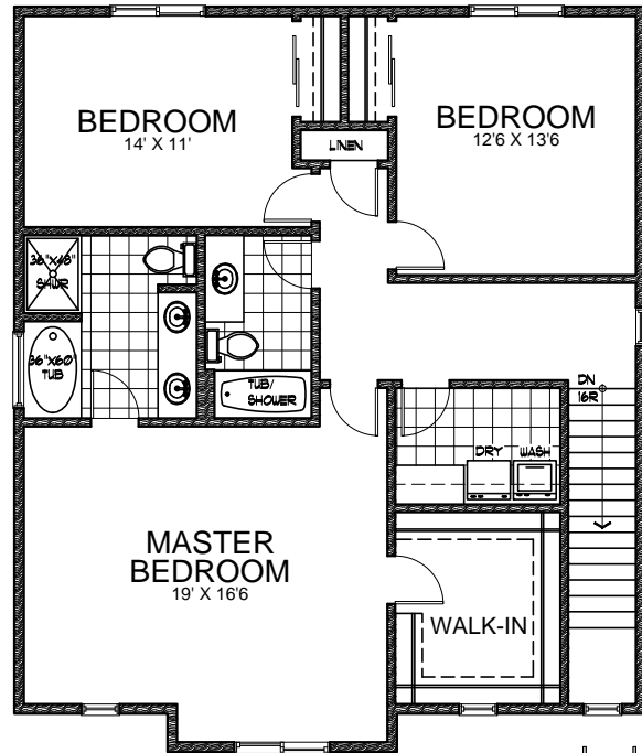
Second Floor 1177 sq ft
