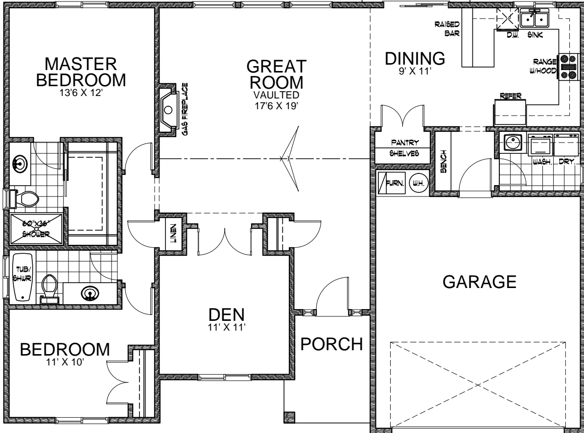
Main Floor 1495 sq ft
