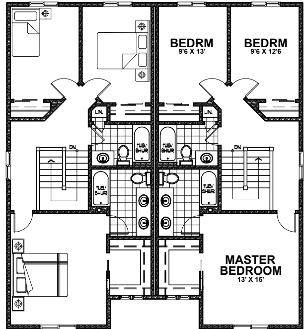
Second Floor 800 sq ft
