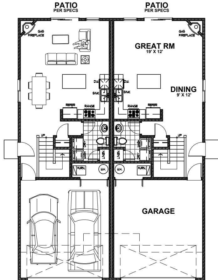
Main Floor 660 sq ft
