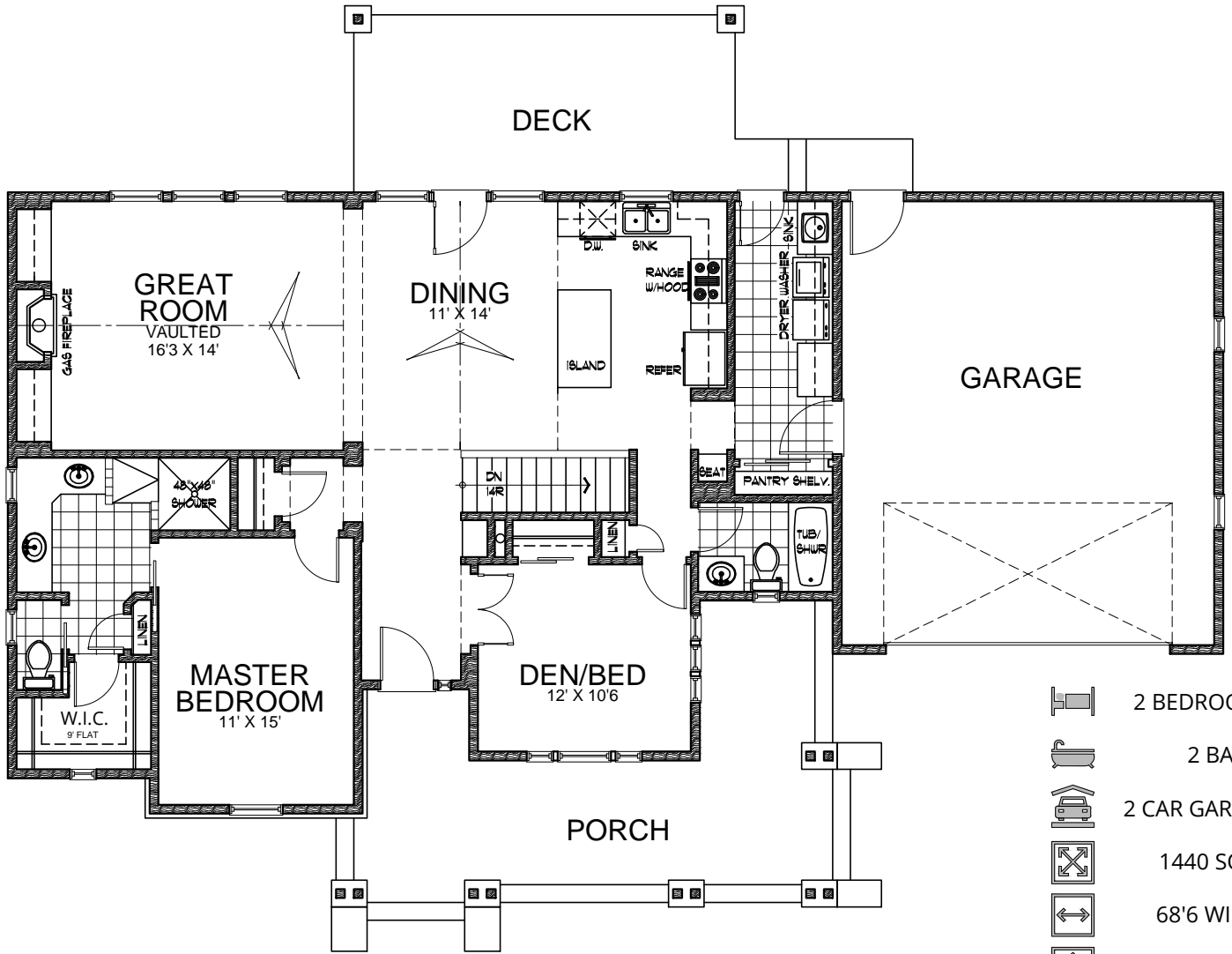
Main Floor 1440 sq ft
