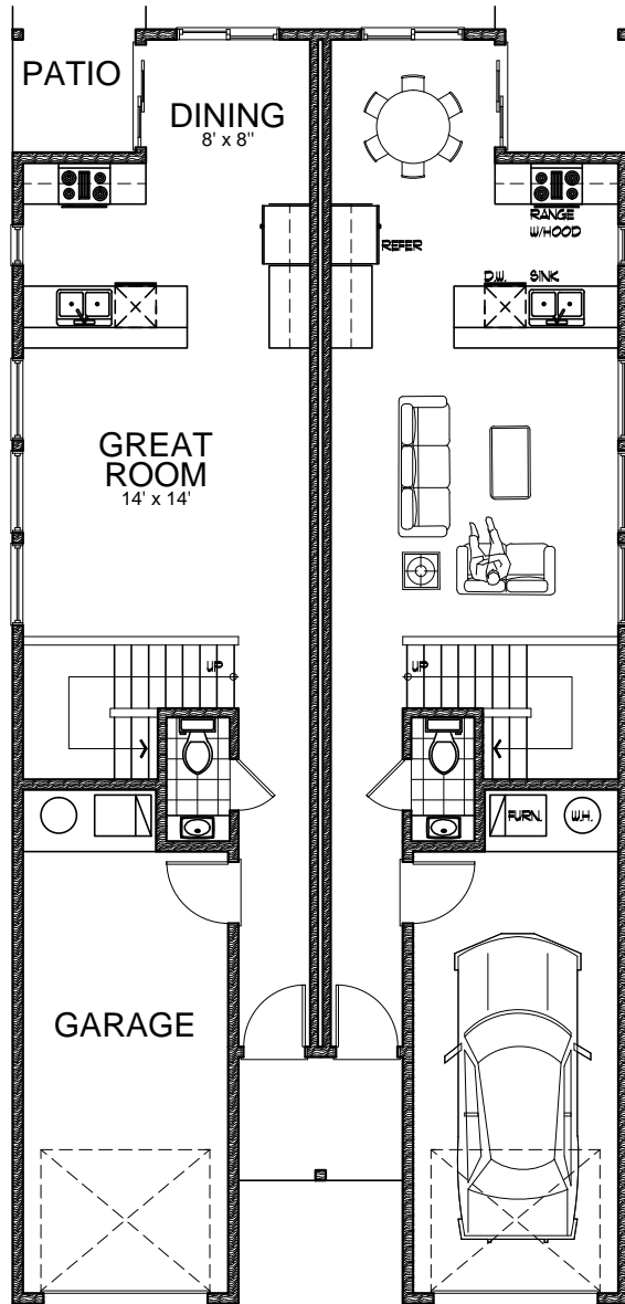
Main Floor 588 sq ft
