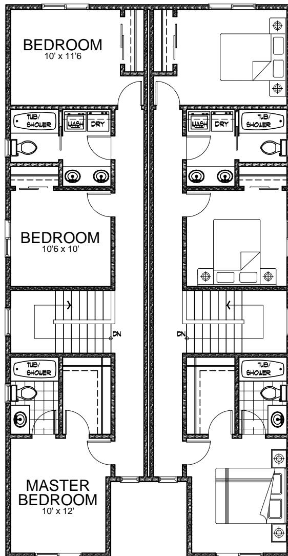
Second Floor 838 sq ft
