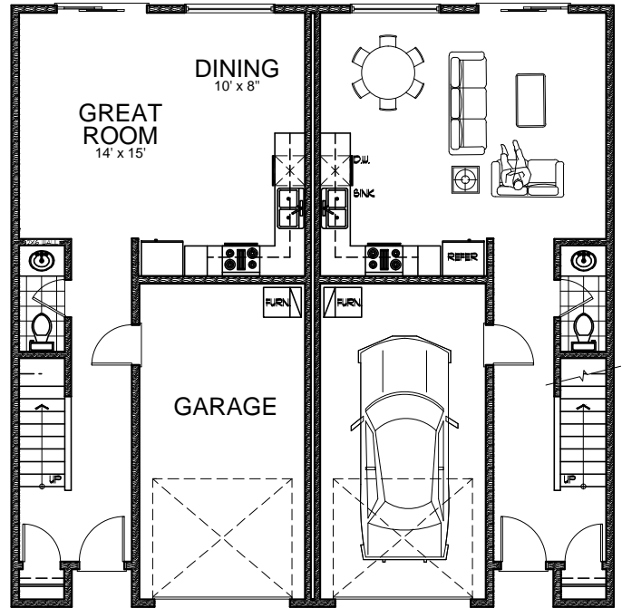
Main Floor 541 sq ft
