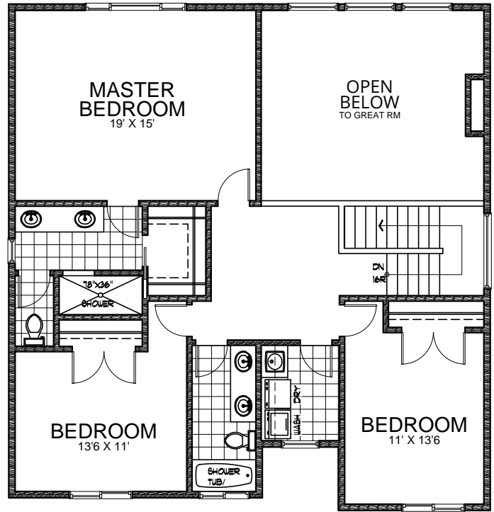
Second Floor 1116 sq ft
