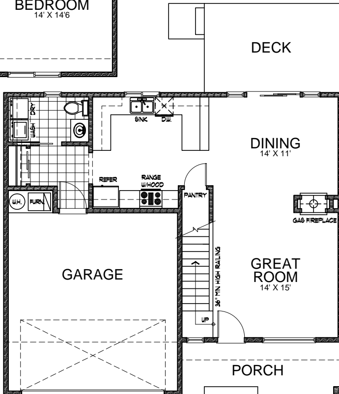
Main Floor 774 sq ft
