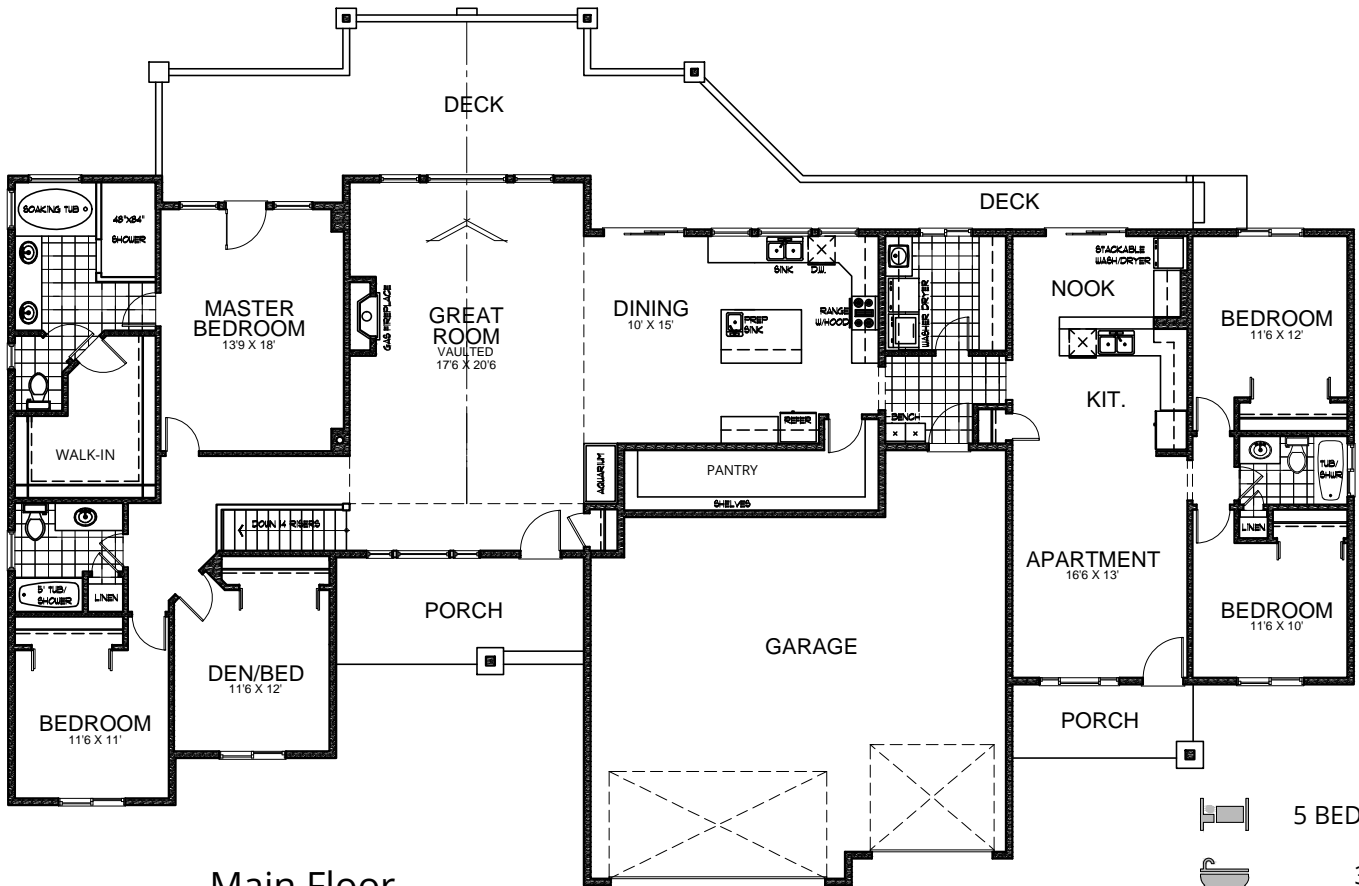
Main Floor 3121 sq ft
