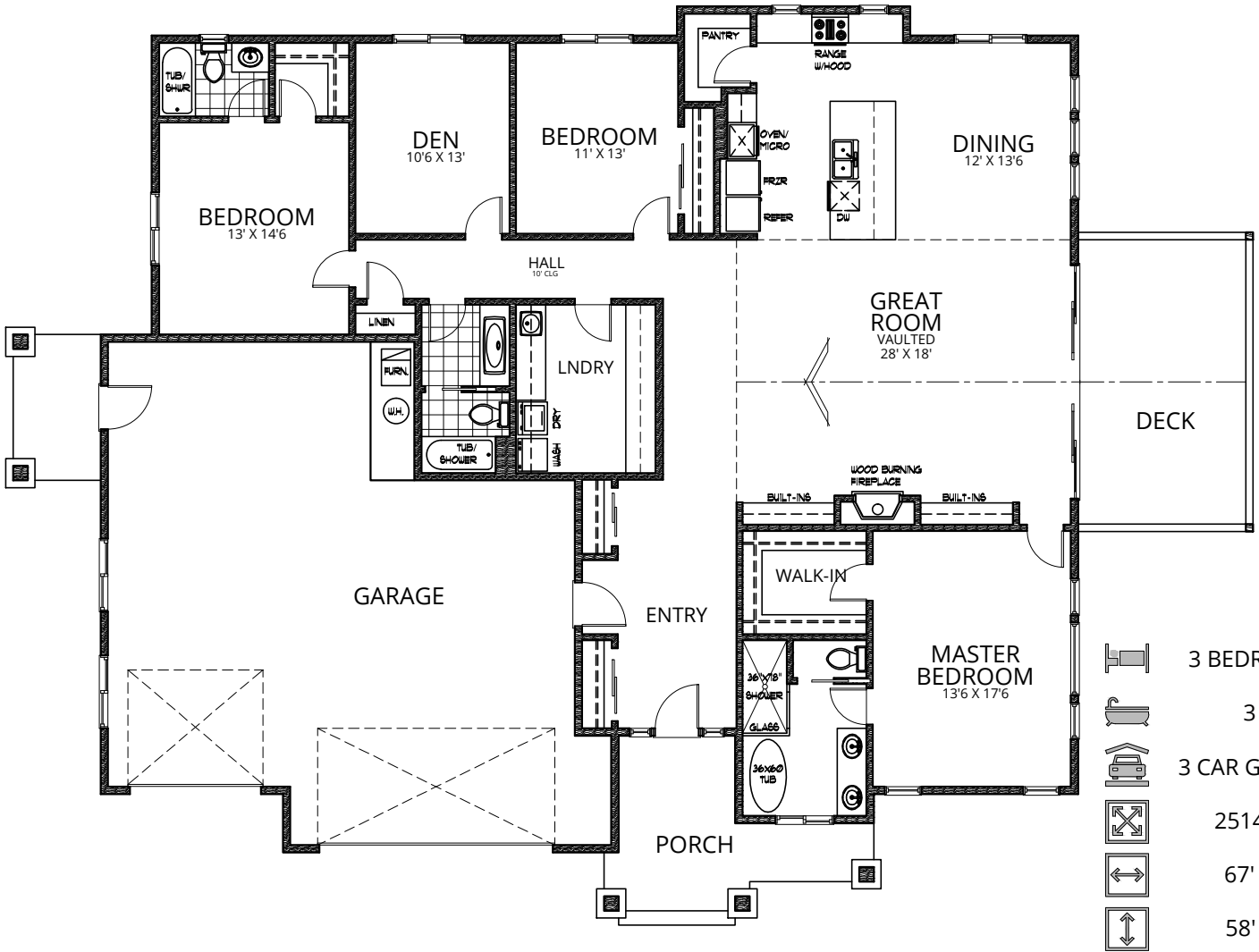
Main Floor 2514 sq ft
