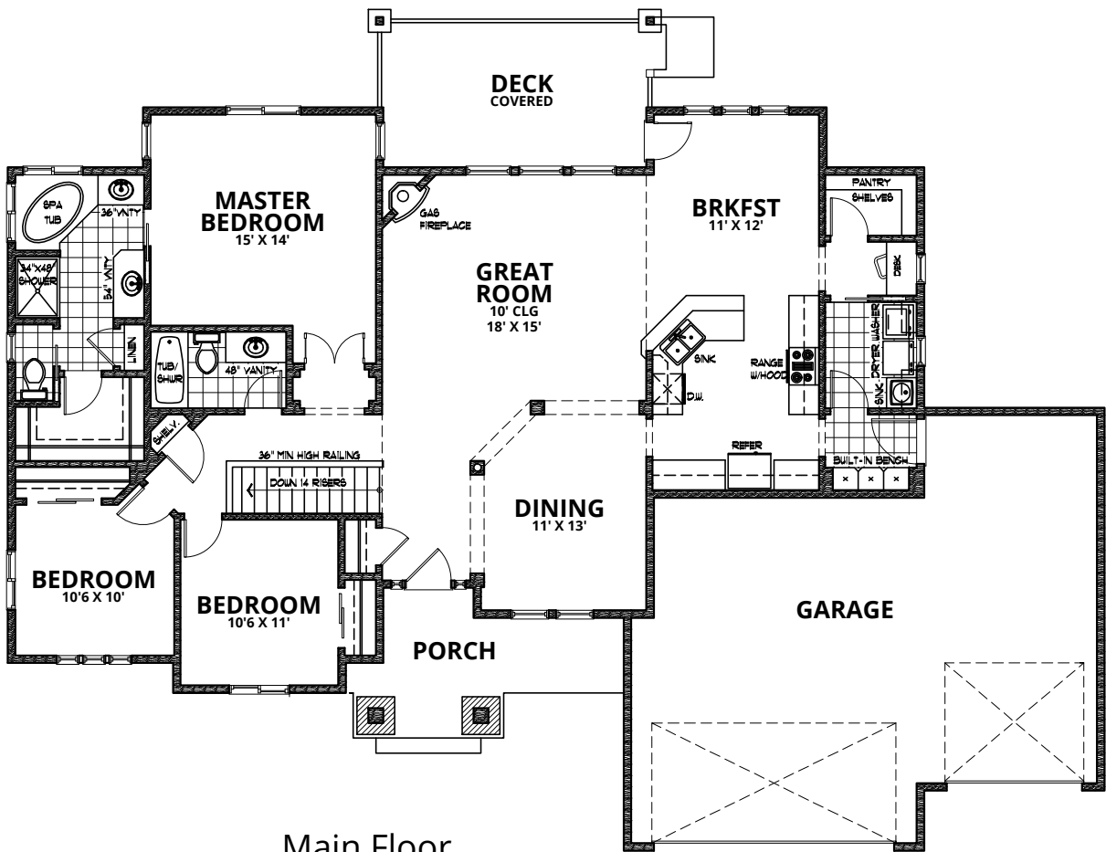
Main Floor 1884 sq ft
