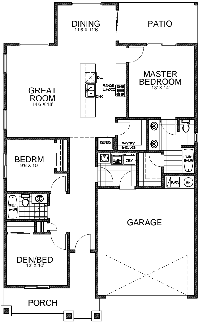
Main Floor 1489 sq ft
