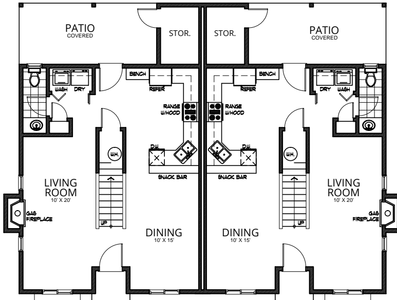
Main Floor 647 sq ft
