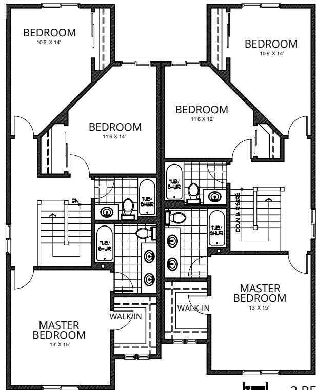
Second Floor 864 sq ft
