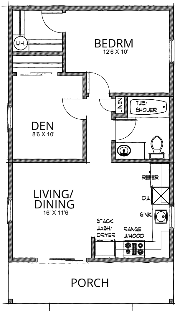
Main Floor 620 sq ft
