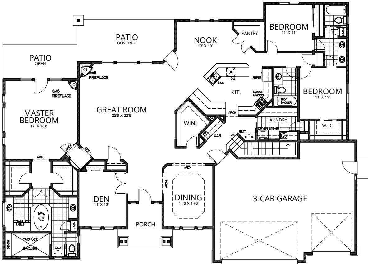
Main Floor 3156 sq ft
