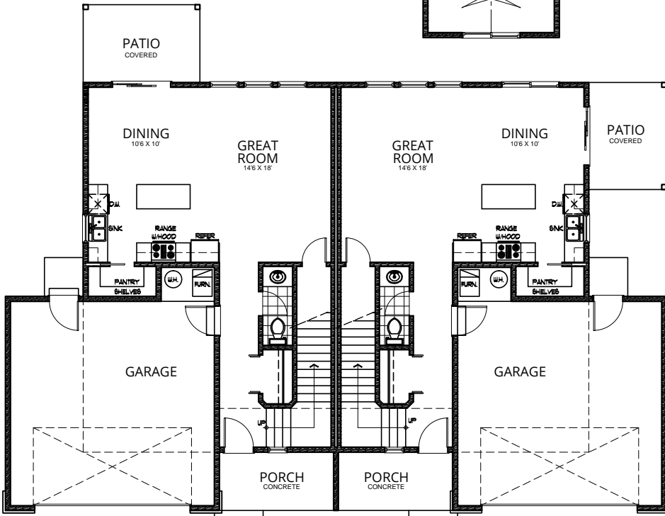
Main Floor
