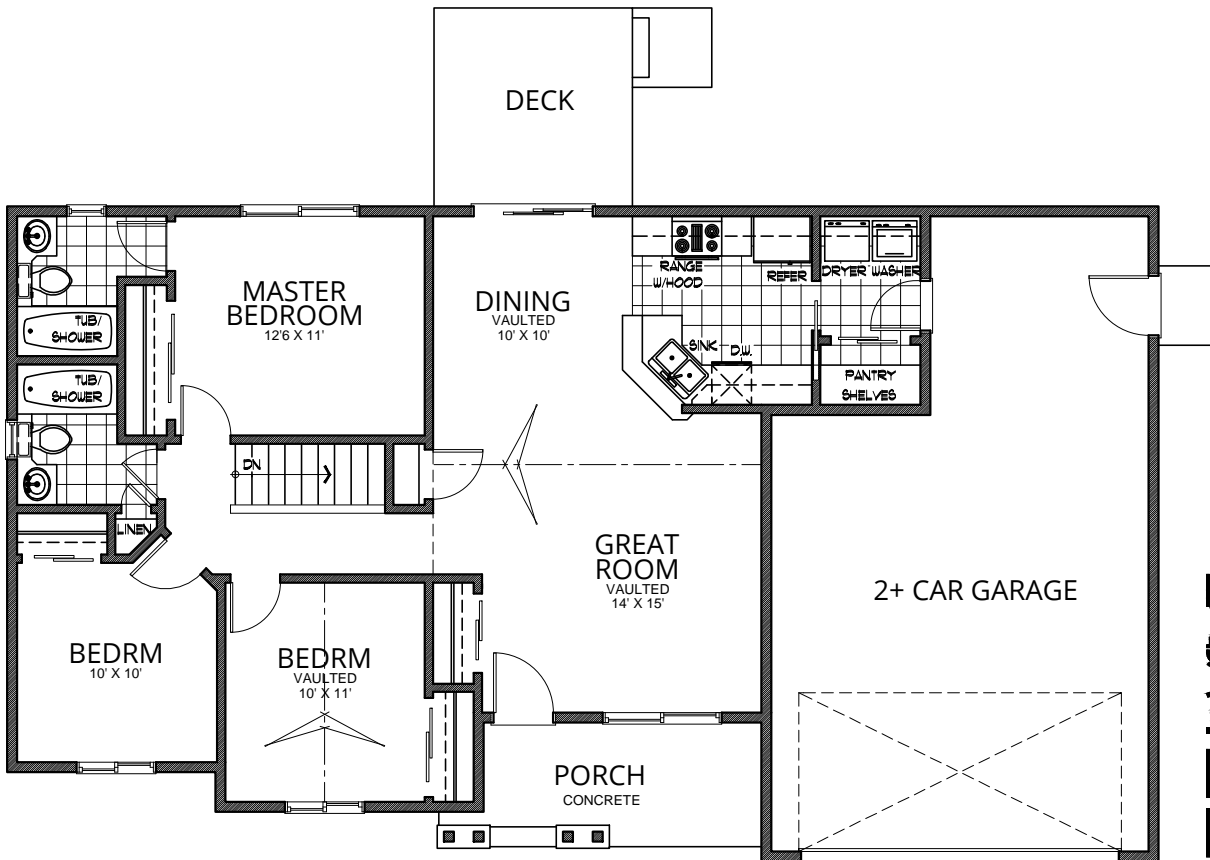
Main Floor 1164 sq ft
