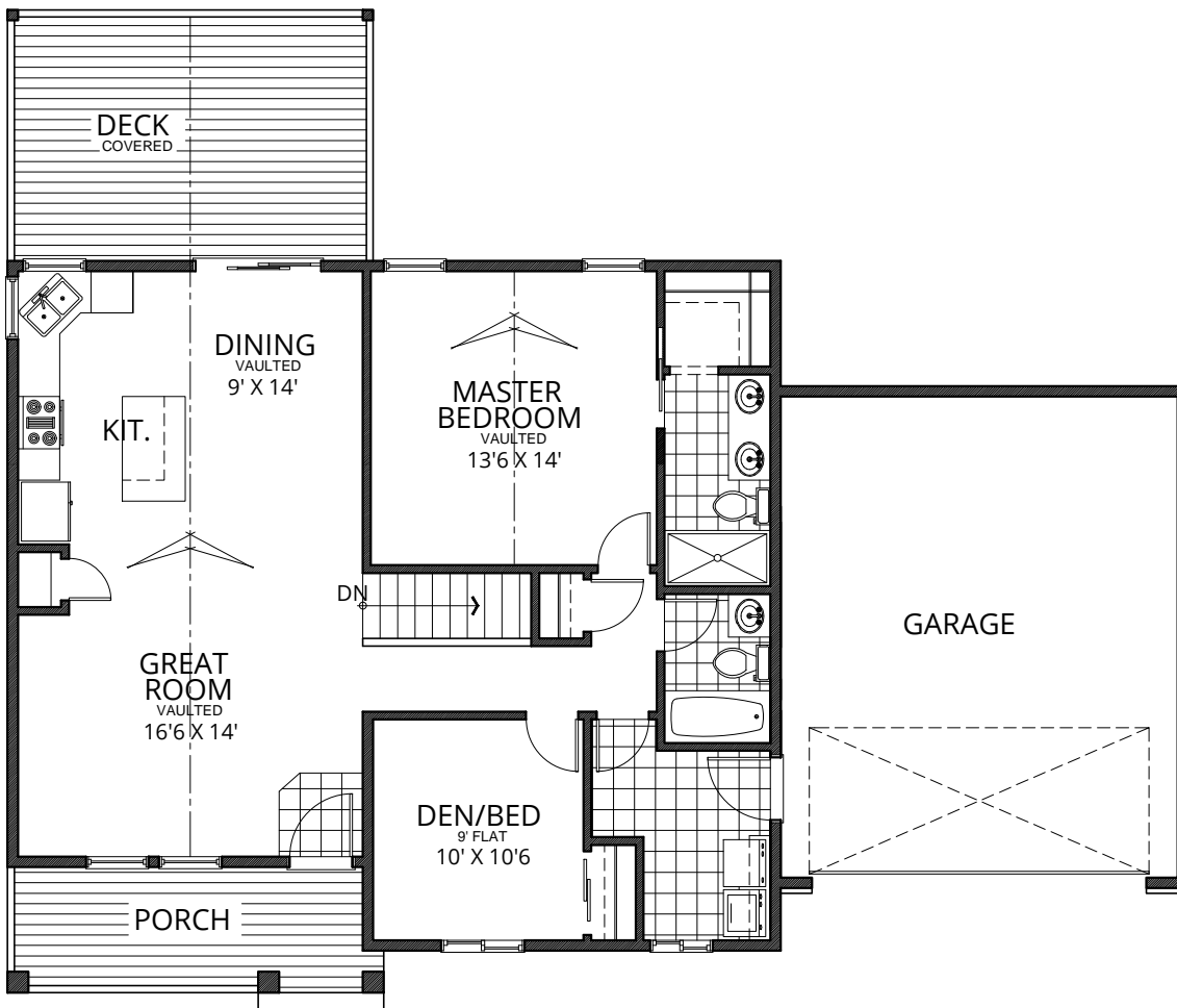
Main Floor 1153 sq ft
