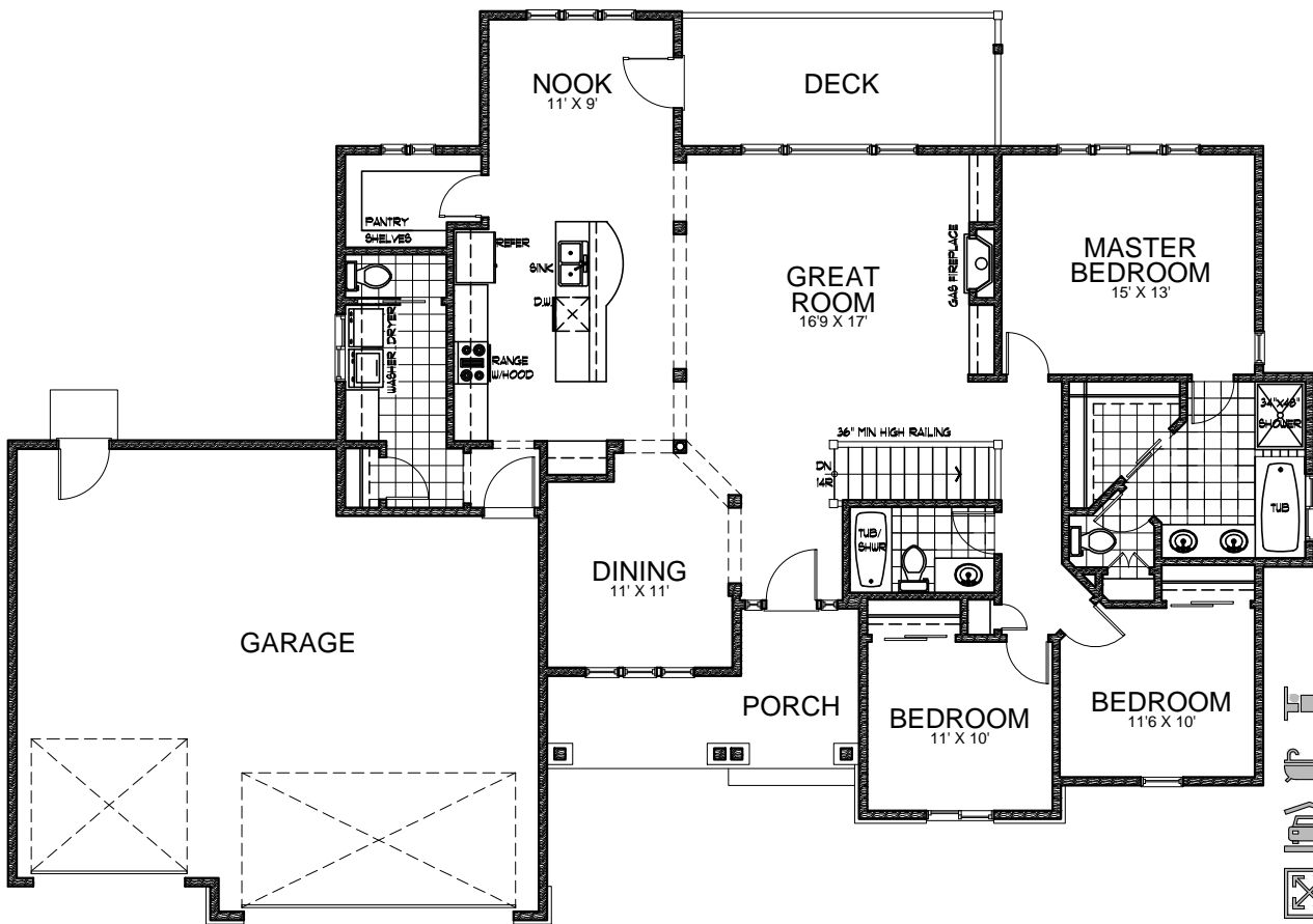
Main Floor 1901 sq ft
