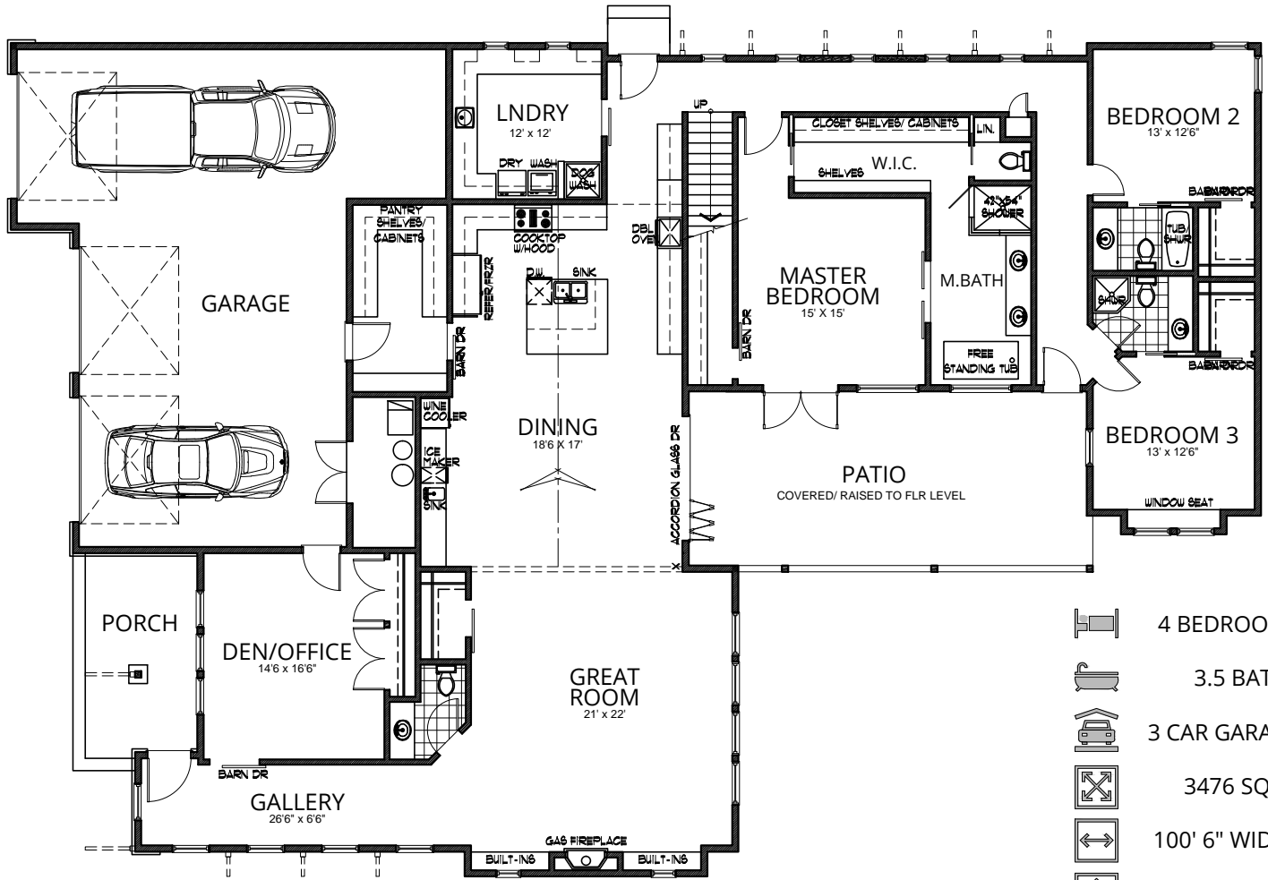
Main Floor 3476 sq ft
